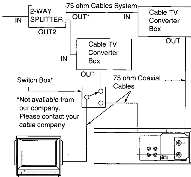
To the 75 ohm VHF input on the TV set
